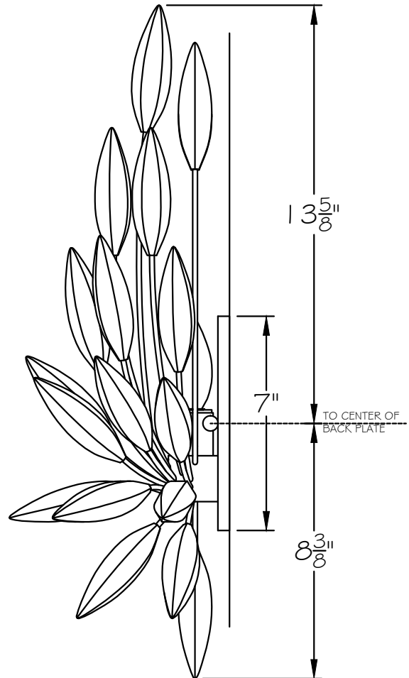
SIDE VIEW
